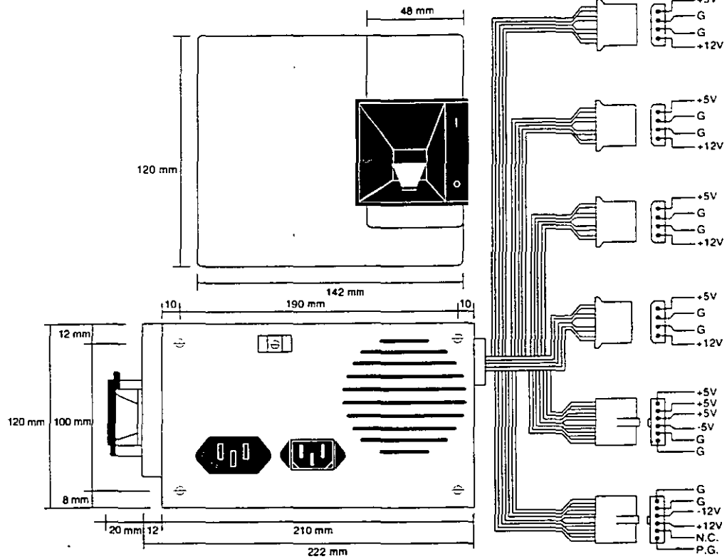
PC/XT-form factor power supply
