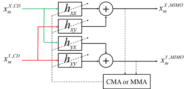
Figure 2.16 Structure of the adaptive time domain MIMO equalizer (TDE-MIMO).
