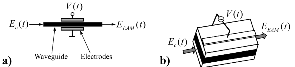
Figure 2.3 a) Schematic representation of an EAM, b) 3D representation of an EAM.
