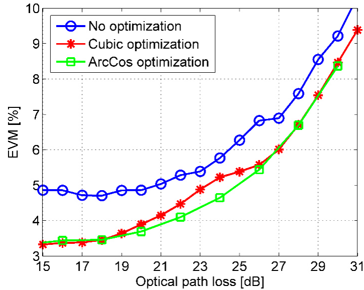
Figure 3.17 Comparison of the EVM as a function of the OPL obtained with different non-linear compensation procedures.
