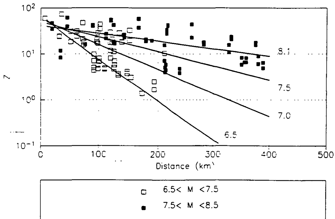
Fig. 6 Parameter Z vs distance, R. Full lines show mean values of Z for several magnitudes, M.
