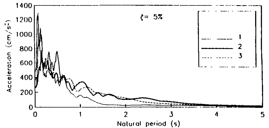
Linear response spectra
