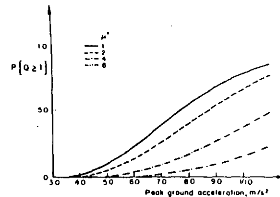
FIG. 5. Failure Probabilities of Single-Story Frames Designed for Different Ductility Factors ( V_{\mu} = 0.5 )
