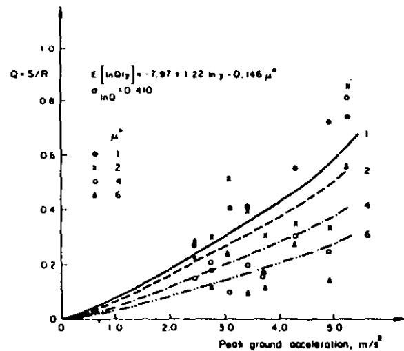
FIG. 3. Normalized Response of Single-Story Frames ( T = 0.36 s and V_{\mu} = 0.5 )
