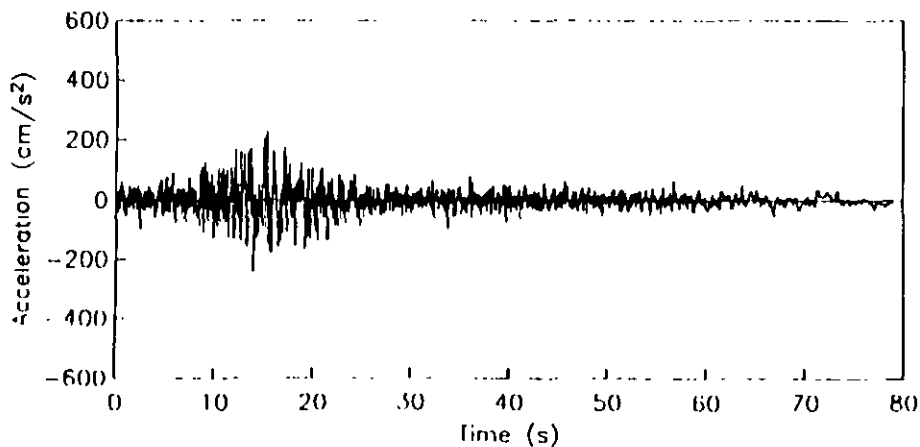
Simulated accelerogram 5
