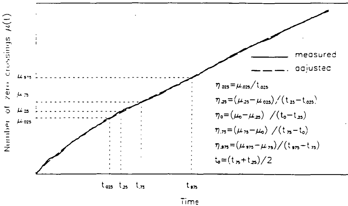
Fig. 1b Number of zero crossings function of ground-motion accelerogram.
