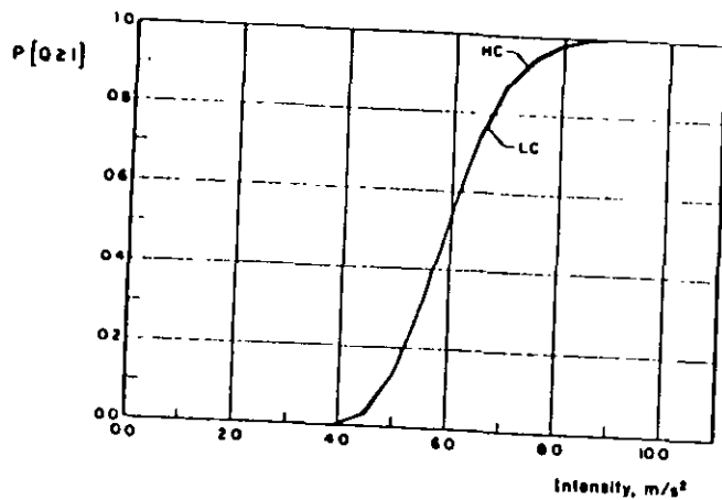
FIG. 7. Failure Probabilities of Three-Story Frames ( T = 0.36 s, \mu^* = 4 , and V_\mu = 0.3 ); High (HC) and Low (LC) Spatial Correlation
