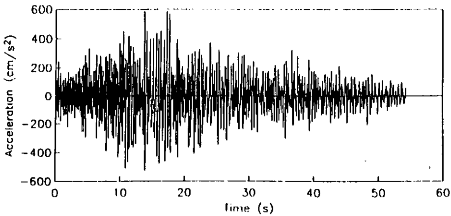
Simulated accelerogram 5
