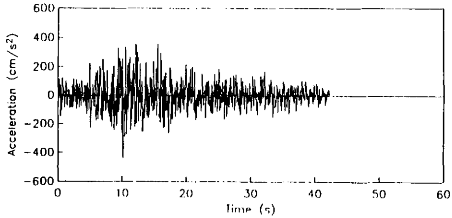
Simulated accelerogram 1
