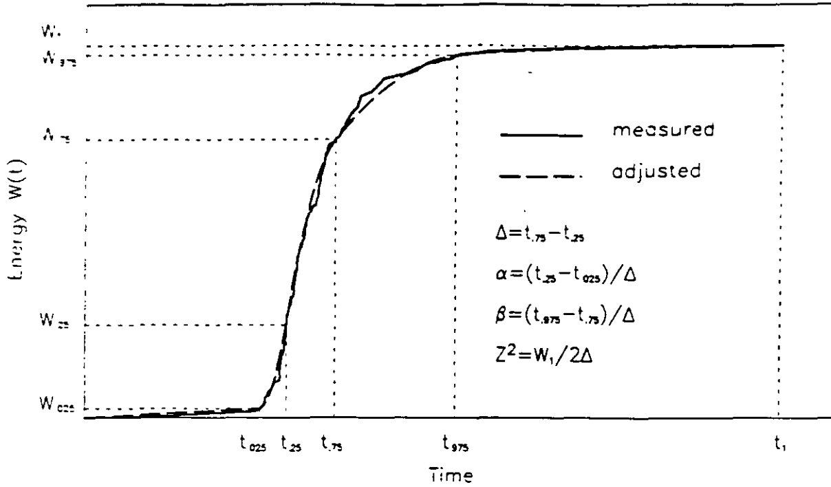
Fig. 1a Energy function of ground-motion accelerogram.
