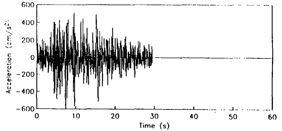
Simulated accelerogram 3
