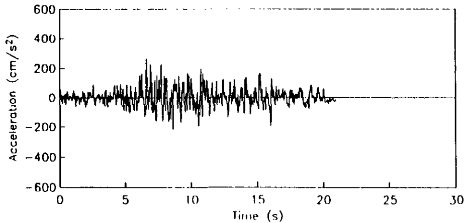
Simulated accelerogram 2
