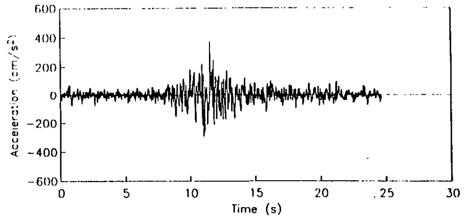
Simulated accelerogram 3
