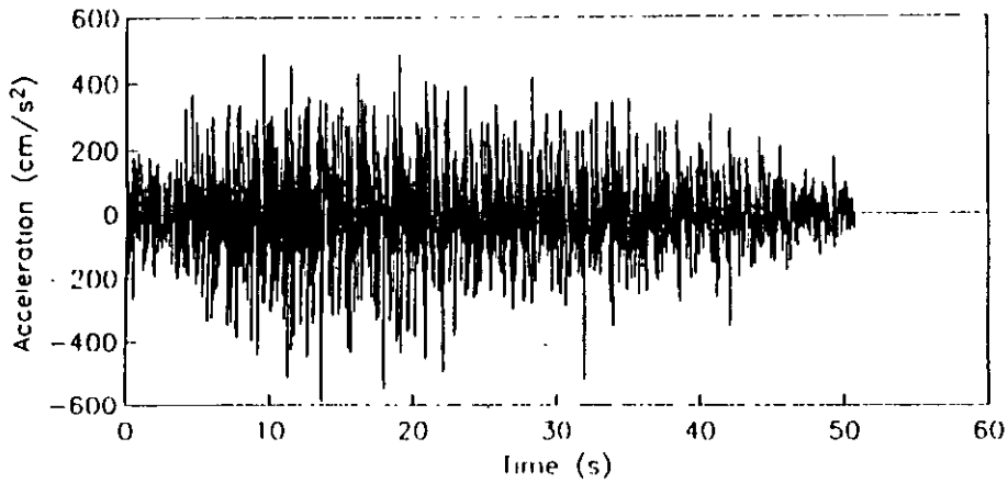
Simulated accelerogram 4
