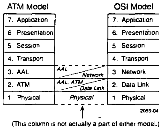
Figure 2-4 ATM and OSI Models
