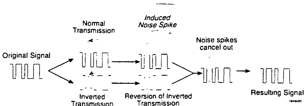
Figure 11-5. Twisted Pair Signal Equalization
