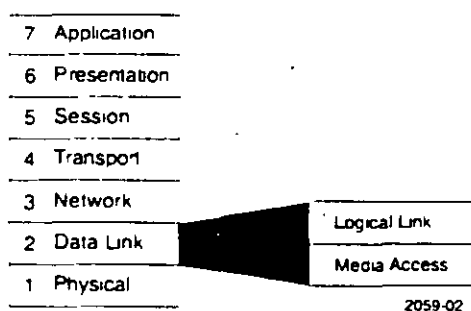
Figure 2-2 Data Link Layer
