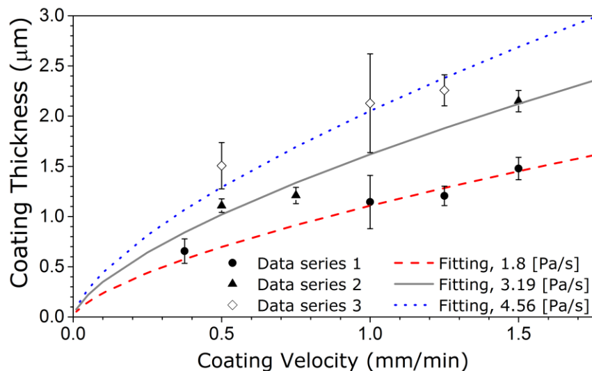
Fig. IV - 10. Characterization of the coating layer thickness for PDMS at different coating velocities and viscosities.
