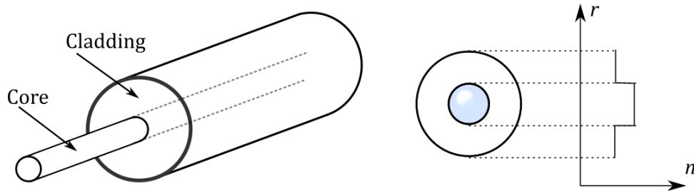
Fig. II - 1. Step-index optical fiber scheme and its refractive index profile.
