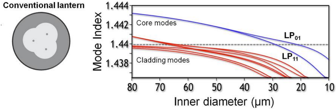
Fig. III - 5. Modal evolution simulations for a PL formed by three identical SMFs. Blue and red lines indicate the modes propagating through the core and the cladding, respectively. Taken from [86].
