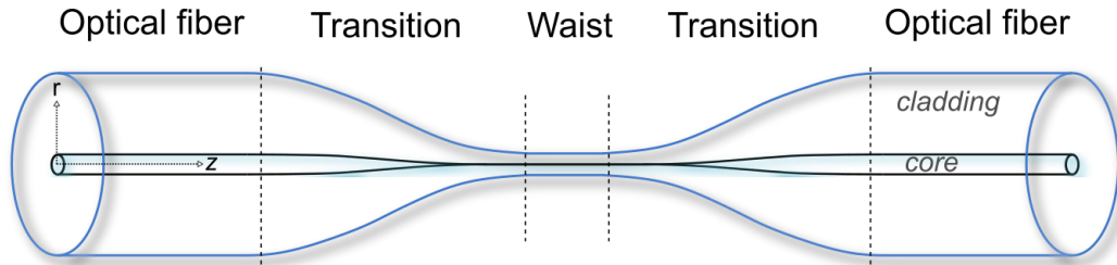
Fig. II - 5. Schematic representation of a tapered optical fiber.
