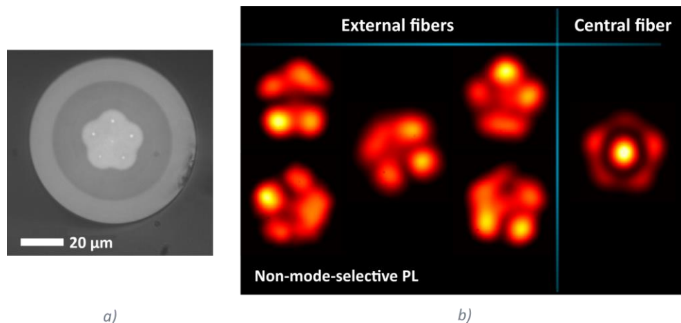
Fig. III - 12. Six fibers photonic lantern. a) End facet cleaved at the waist section. b) Near field mode profiles from a non-mode-selective PL at 1550\ \text{nm} .
