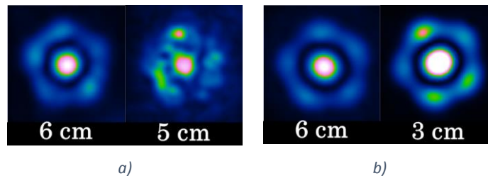
Fig. III - 19. Near-field LP_{02} mode profile from MSPLs with different transition lengths: (a) step-index and (b) graded-index fibers.
