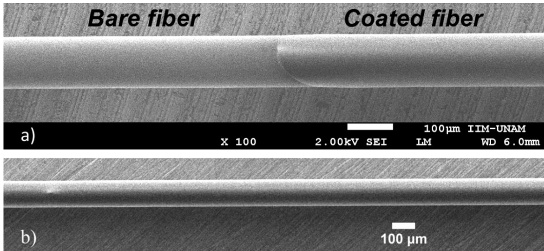
Fig. IV - 8. Scanning electron microscopy (SEM) images of an optical fiber coated with a layer of UVpoly of approximately 1.15 μm at a speed of 1 mm/min: a) initial section of the coating, and b) uniformly coated optical fiber (bright dot caused by sample preparation-manipulation for SEM imaging).
