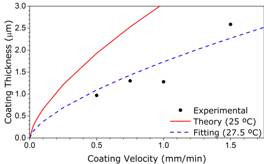
Fig. IV - 9. Measured layer thicknesses for the UVpoly at different coating velocities and calculated thickness for two different temperatures.
