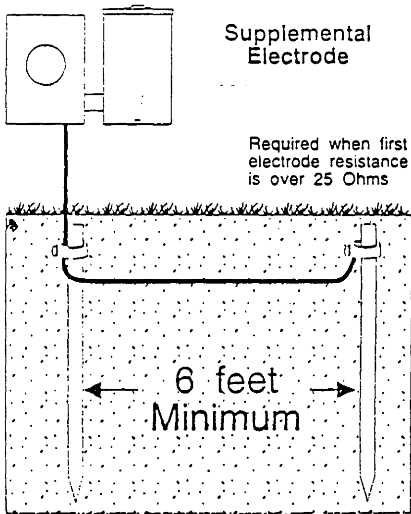
Fig. 12-27 If main electrode is over 25 ohms, supplemental electrode required [250-84].
