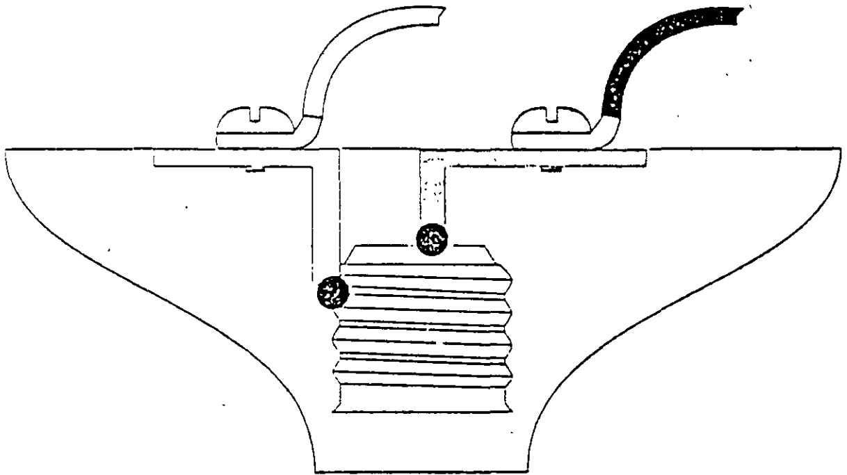
Fig. 4-8 Terminal identification [200-10].
