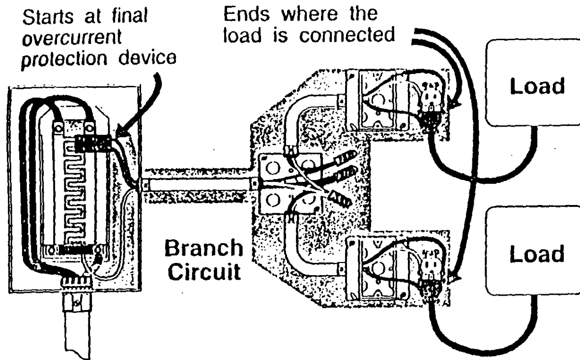
Fig. 2-6 Branch Circuit: Circuit conductor after the final overcurrent protection device.
