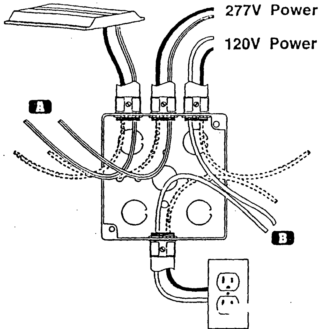
Fig. 4-4 Grounded conductor identification, different systems [200-6(d)]. (A) 277 volt circuit, identified white with color tracer. (B) 120 volt circuit, identified white or gray.
