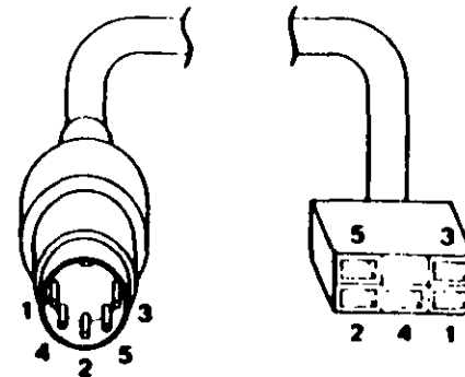
Figure 2. Continuity Check
