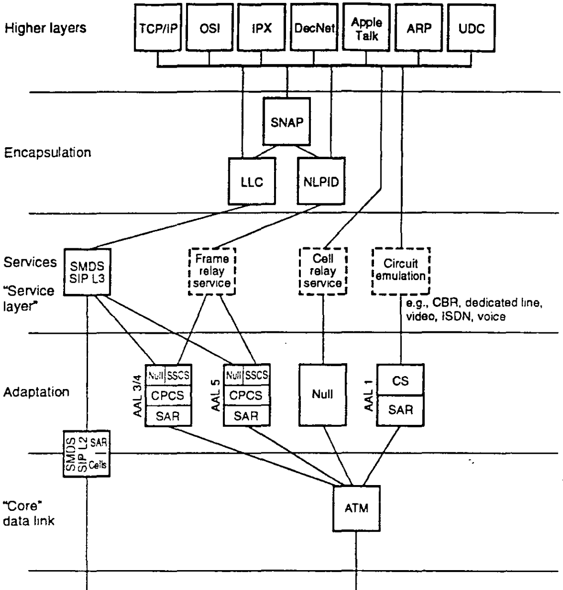
Figure 3.5 Support of user applications. CPCS = common part CS; SSSCS = service-specific CS; LLC = logical link control; SNAP = Subnetwork Access Protocol; NLPID = Network Layer Protocol ID.
