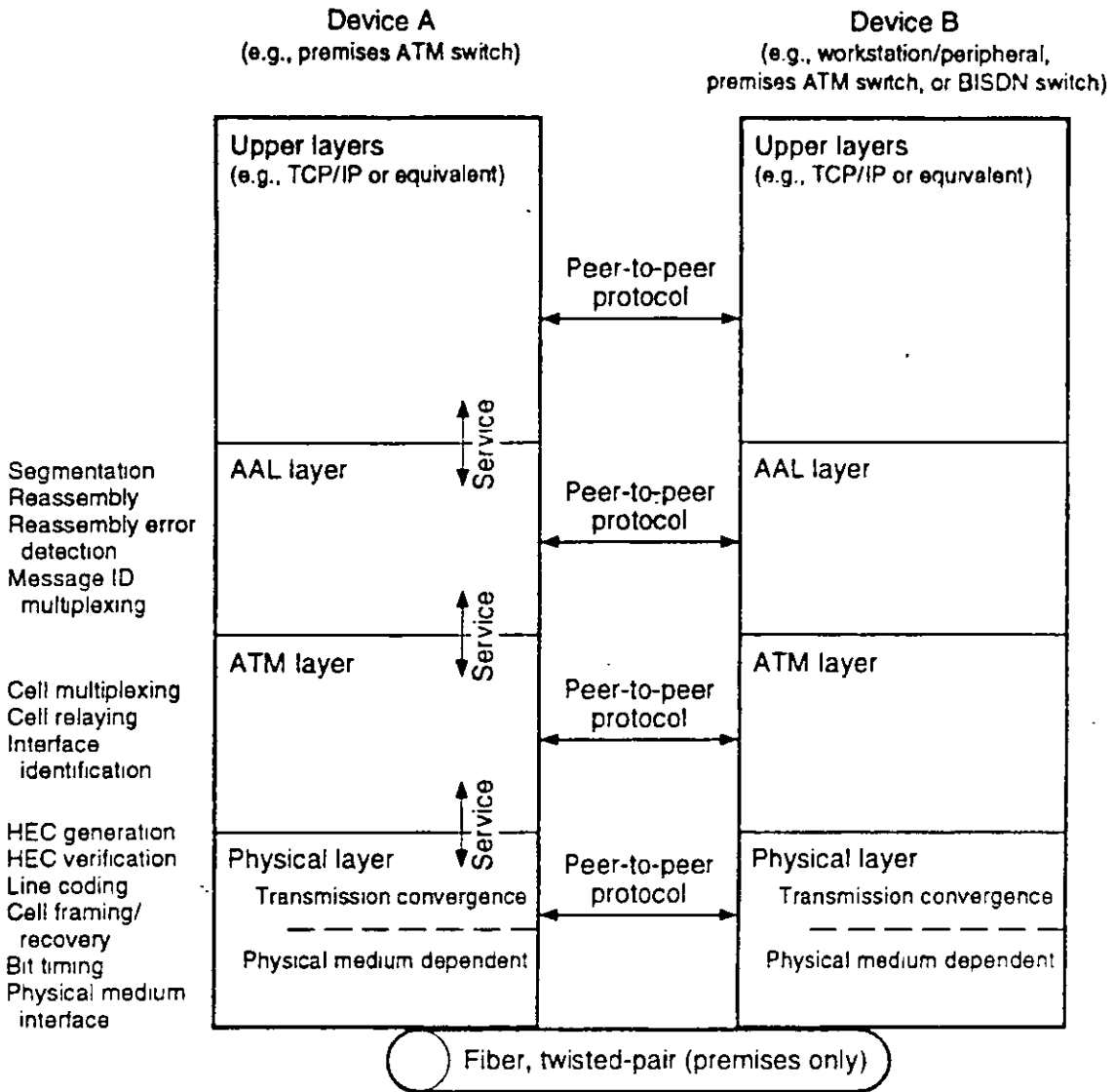
Figure 2.6 ATM protocols.
