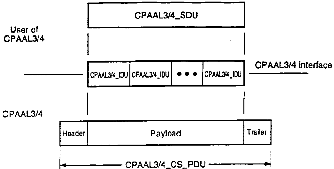
Figure 3.11 Streaming-mode service.
