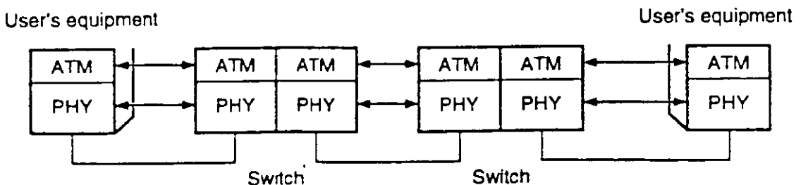
Figure 2.2 Cascaded ATM entities.
