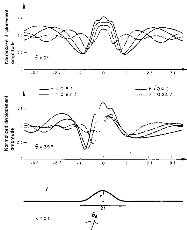
Fig. 6. Normalized displacement amplitudes in a surface of a ridge under incident SH waves. (After Bouchon, 1973)
