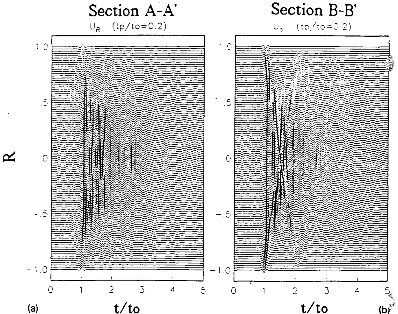
Fig. 18. Horizontal synthetic seismograms in 101 stations along the sections A-A' and B-B', respectively, of the three-dimensional model.
