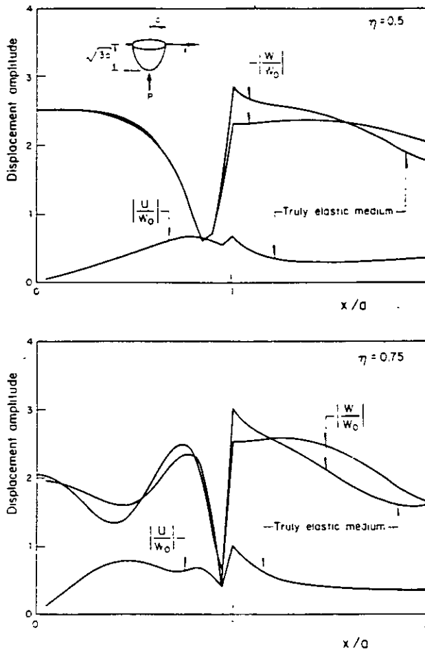
Fig. 5. Displacement amplitudes in a semi-ellipsoidal surface cavity under vertical incidence of P waves. Vertical displacements are computed for a restricted elastic medium in which horizontal motion is restricted. Comparison is provided with computations for a truly elastic medium
