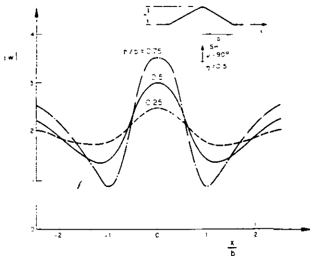
Fig 10 Displacement amplitudes at the free-surf. Ridges with different aspect ratio h/b . Vertical incidence of SH waves with normalized frequency \eta=0.5
