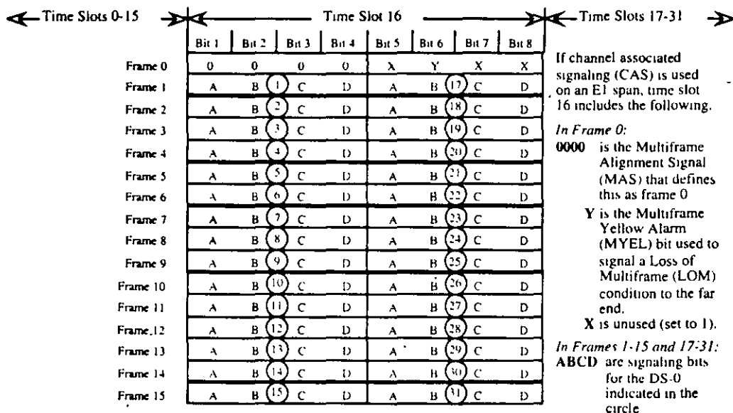
E1 CAS Signaling Multiframe Structure in Time Slot 16
