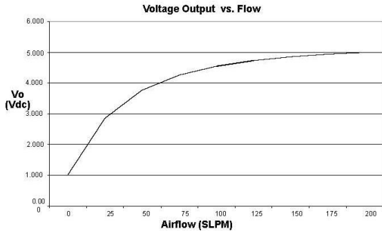
Figure 1. Voltage Output vs. Airflow
