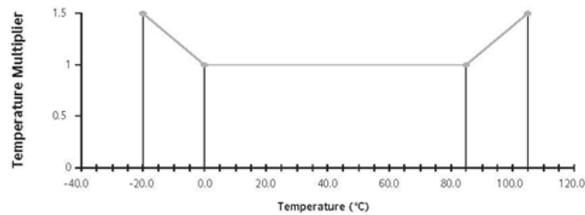
Error Band Multiplier Over -20^\circ\text{C} to +105^\circ\text{C}
