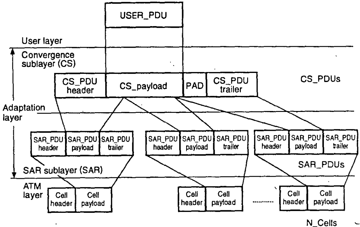
Figure 3.9 Adaptation Layer model for bursty data services.
