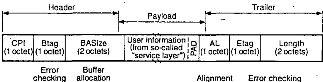
Figure 3.13 CPAAL3/4_CS_PDU Sublayer format of AAL.
