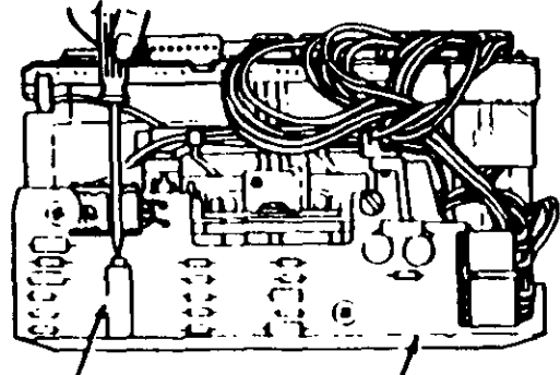
Variable Resistor Servo Board
