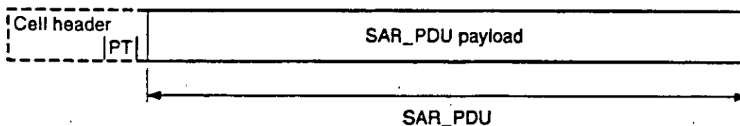
Figure 3.18 SAR_PDU format for AAL5. [Note: The payload type (PT) field belongs to the ATM header. It conveys the value of the AUU parameter end-to-end.]
