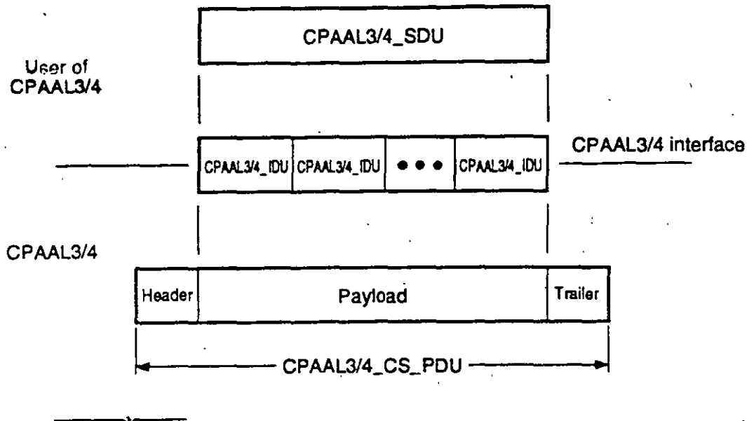
Figure 3.11 Streaming-mode service.
