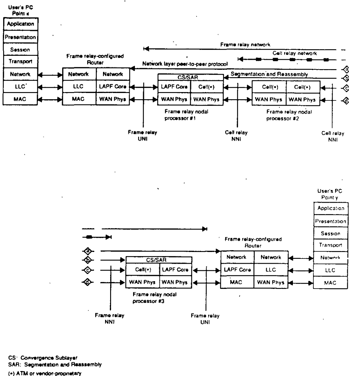
Figure 11.7 Protocol stacks in a frame relay/cell relay network.
