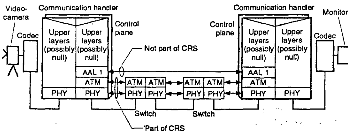
Figure 1.16 Example of video application over ATM/cell relay arrangement.
