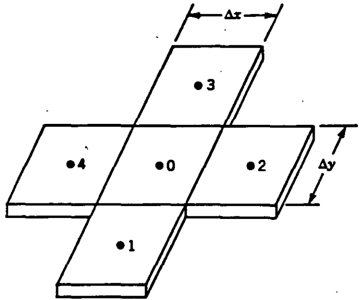
Block-centered grid.
