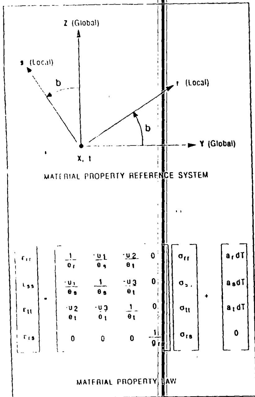
Figure X-21 ASOLID Element Material Properties
