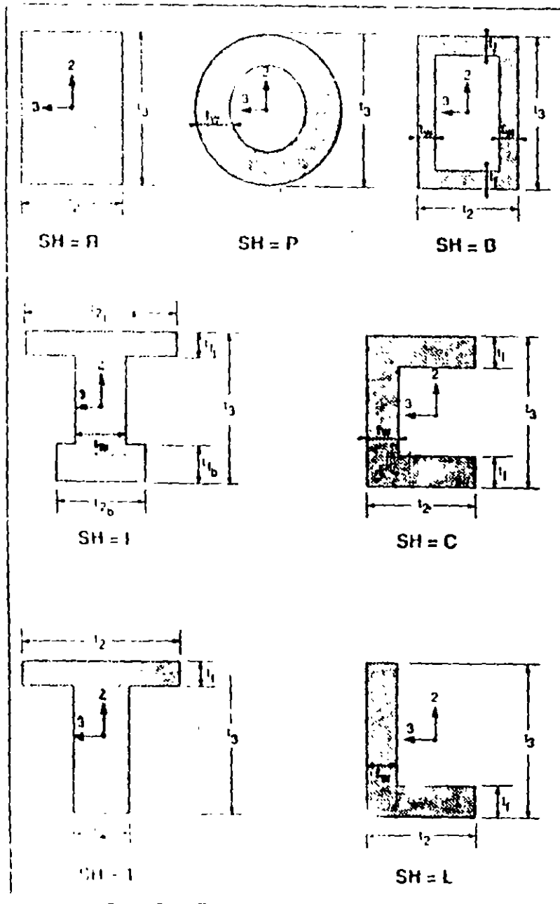
Figure X-9 Automatic Section Property Calculation
