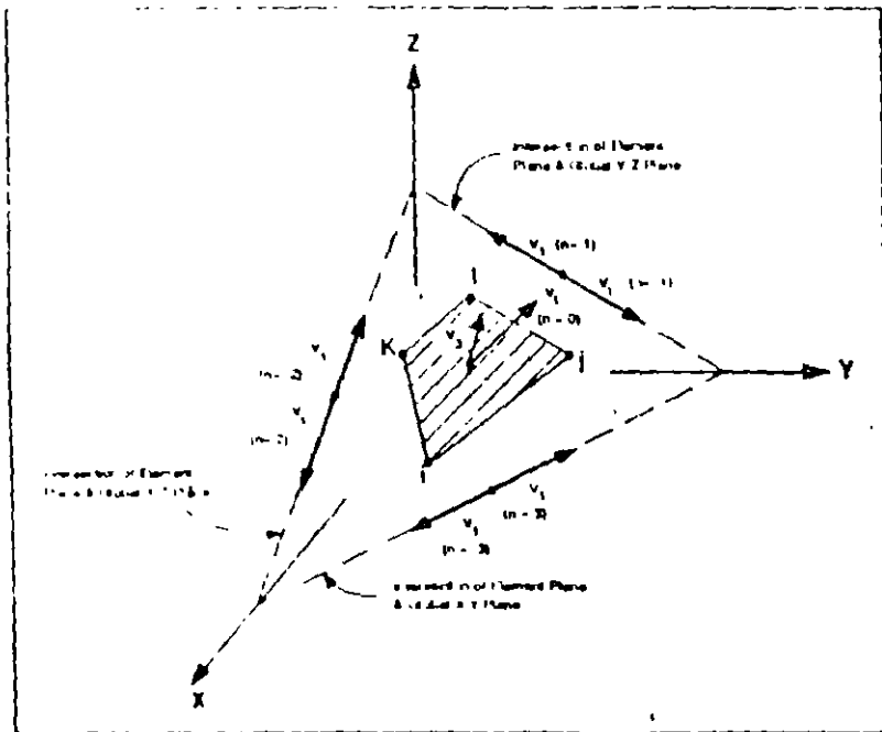
Figure X-18 Shell Element Local Axis
