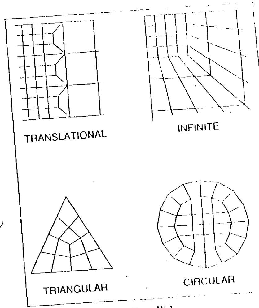
Figure IV-2 Finite Element Mesh Examples and Mesh Transitions Using 4-Node Elements
