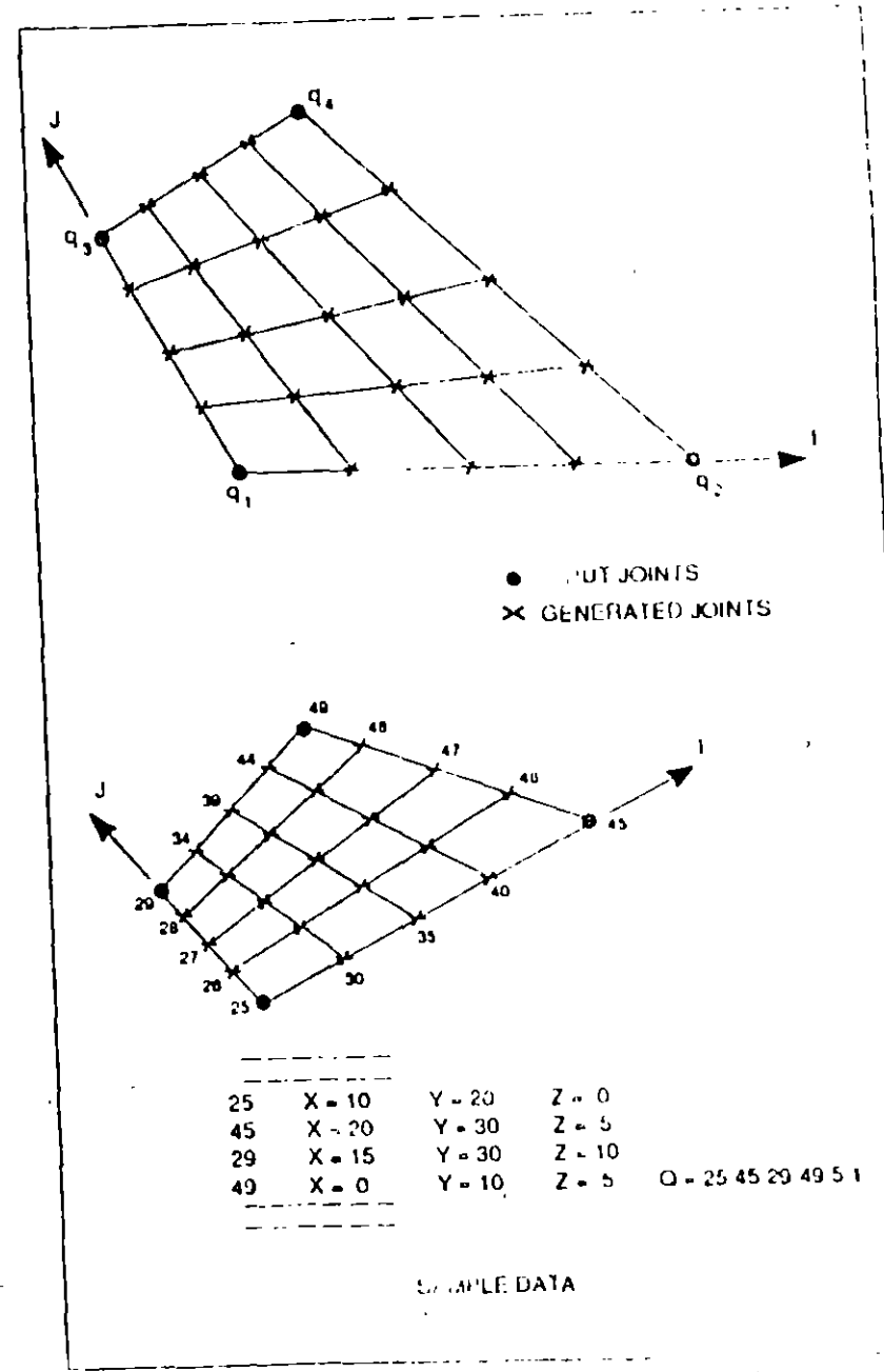
Figure X-2 Quadrilateral Joint Generation
