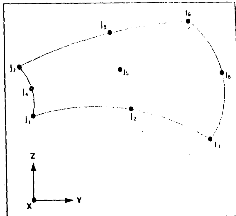
Figure X-22 Variable Three- to Nine-Node Two-dimensional Isoparametric Element
