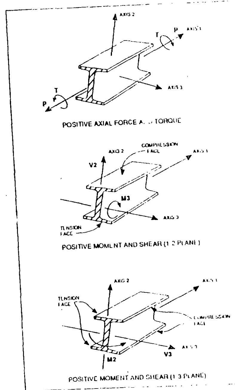
Figure VIII-9 FRAME Element Forces
