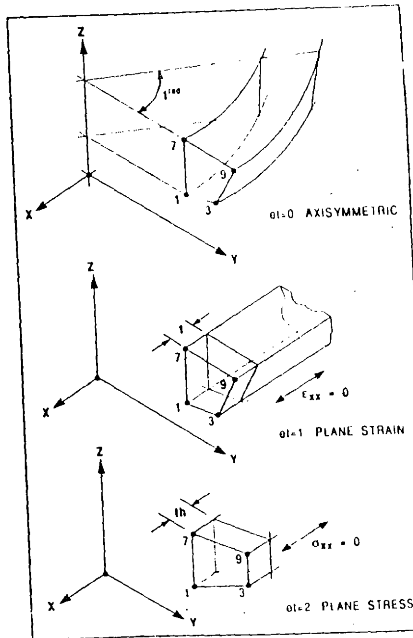
Figure X-20 ASOLID Element Types
