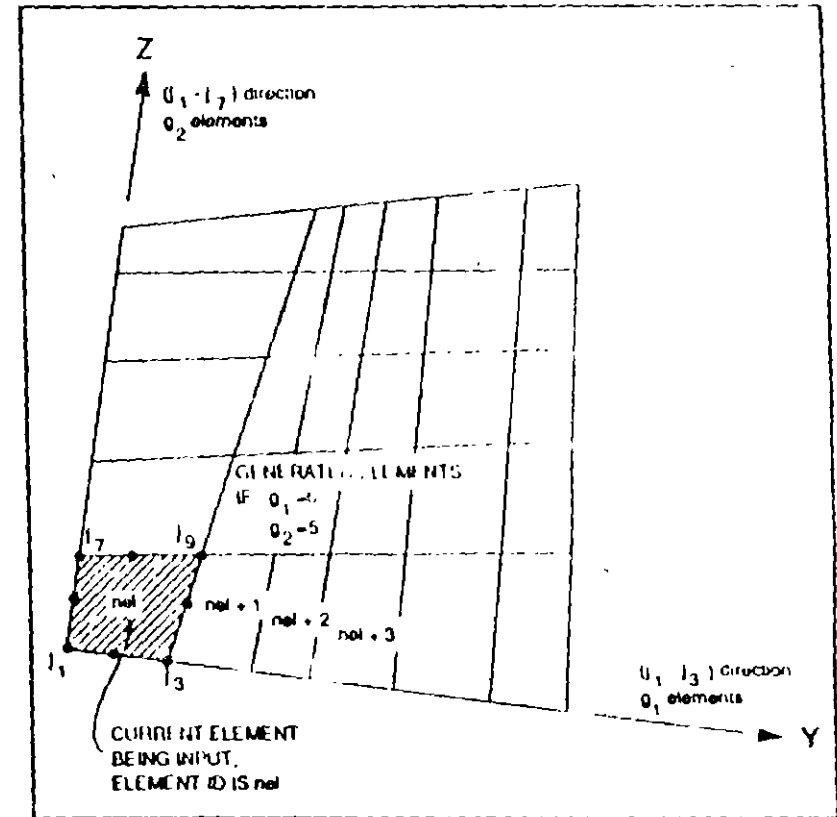
Figure X-23 ASOLID Element Generation
