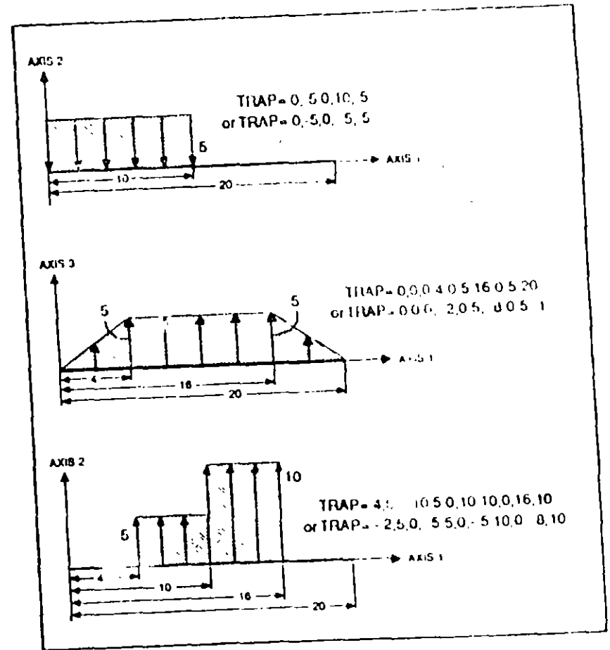
Figure X-13 Trapezoidal Load Examples
