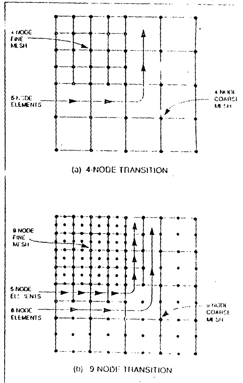
Figure IV-3 ASOLID Element Mesh Transitions
