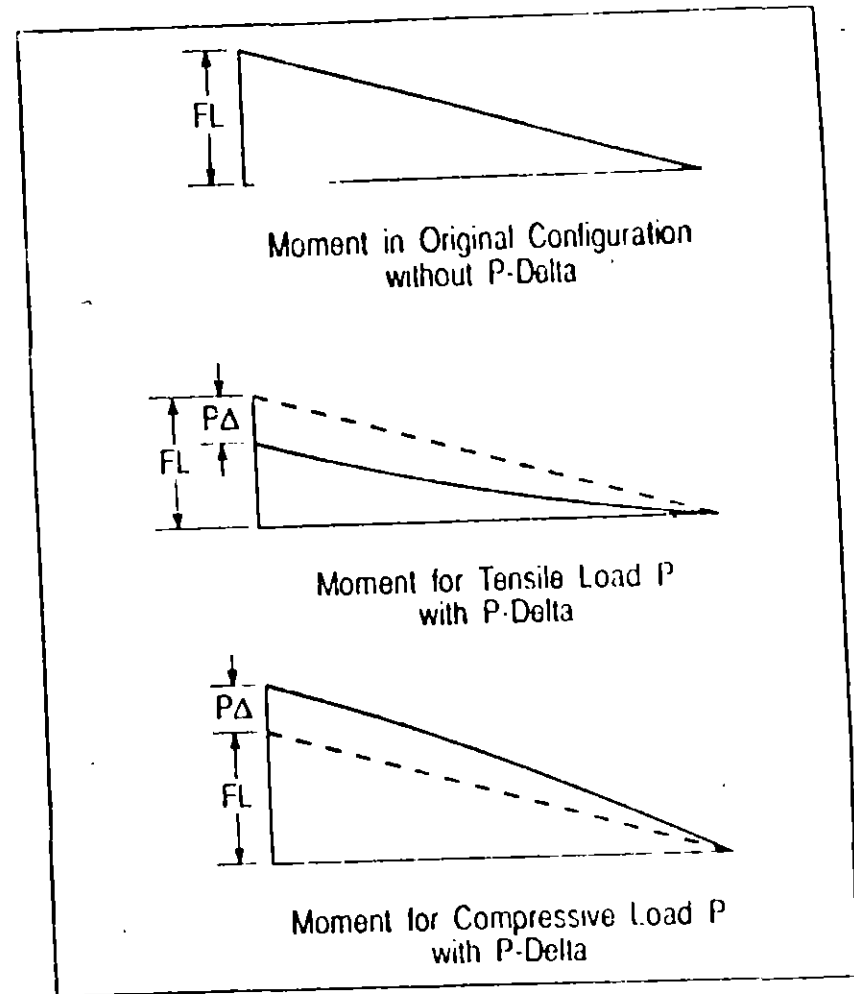
Figure VI-2 Cantilever Beam Example — Moment Diagrams
