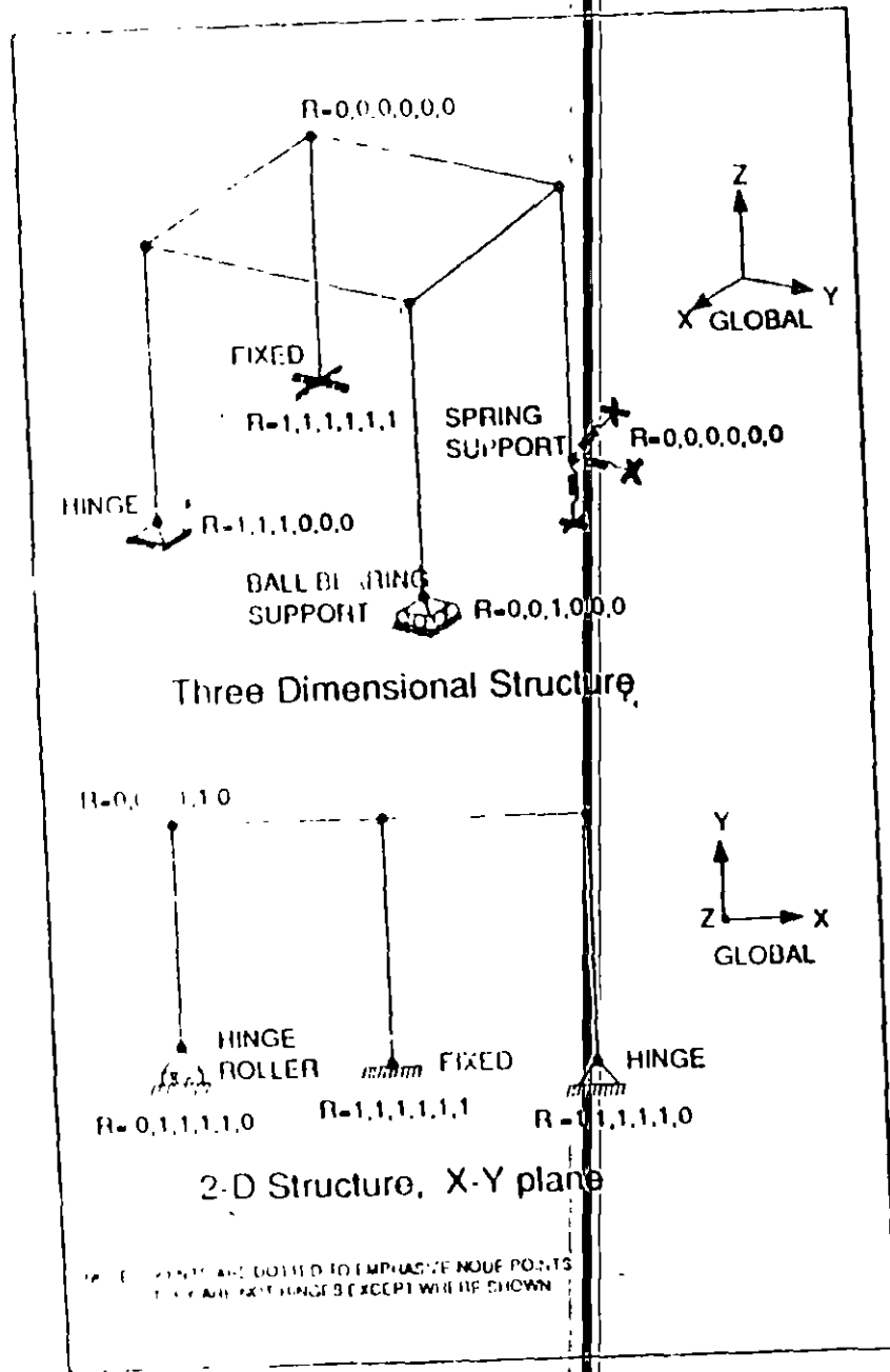
Figure X-6 Examples of Restraint Conditions
