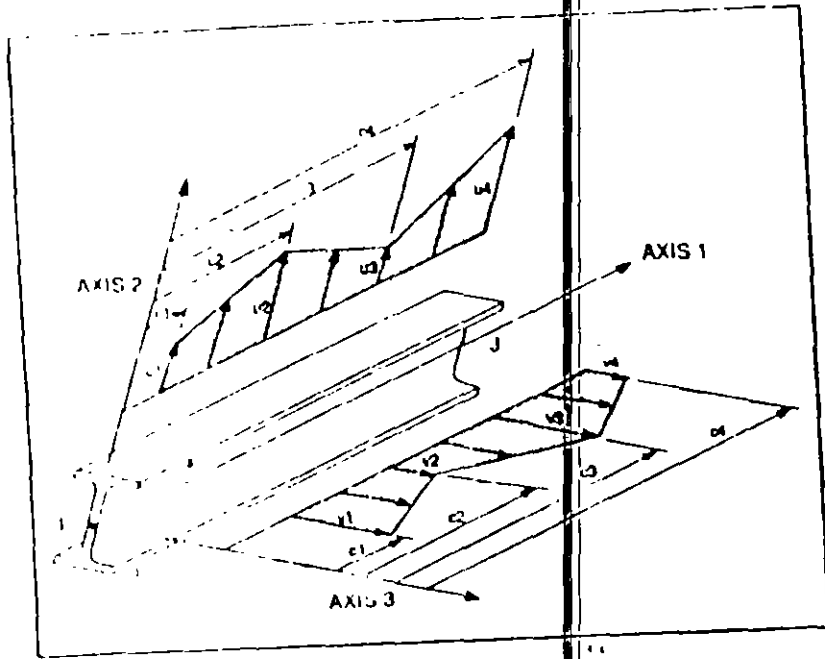
Figure X-12 Definition of Positive Trapezoidal Loads
