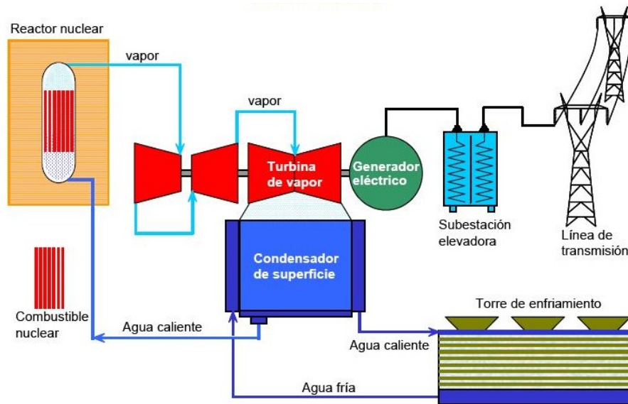
Figura 1.10 Central nucleoelectrica
