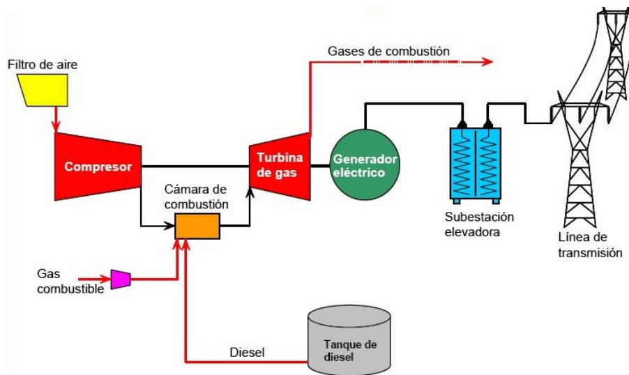
Figura 1.3 Central turbogás
