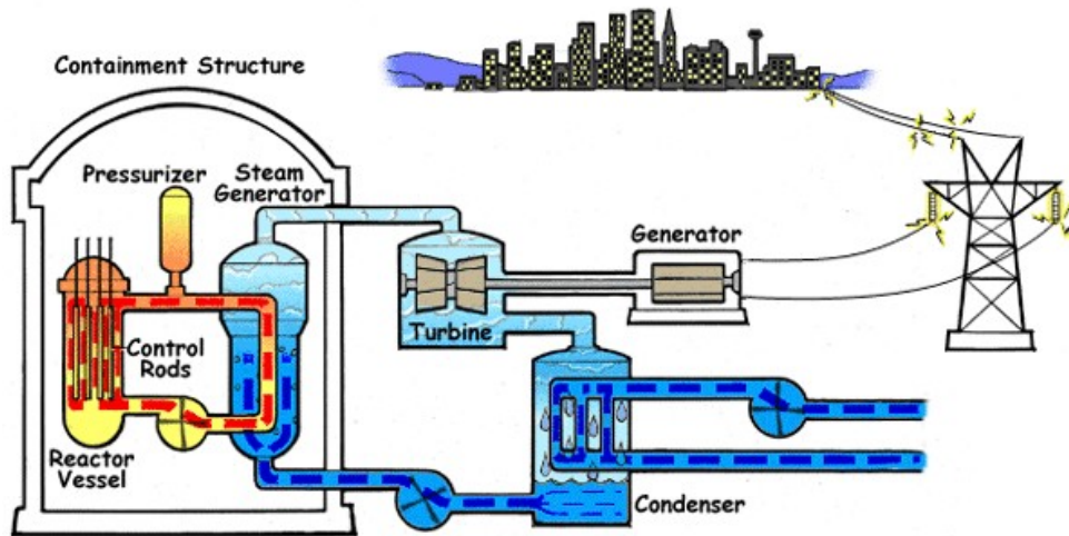
Figura 2.6 Reactor PWR
