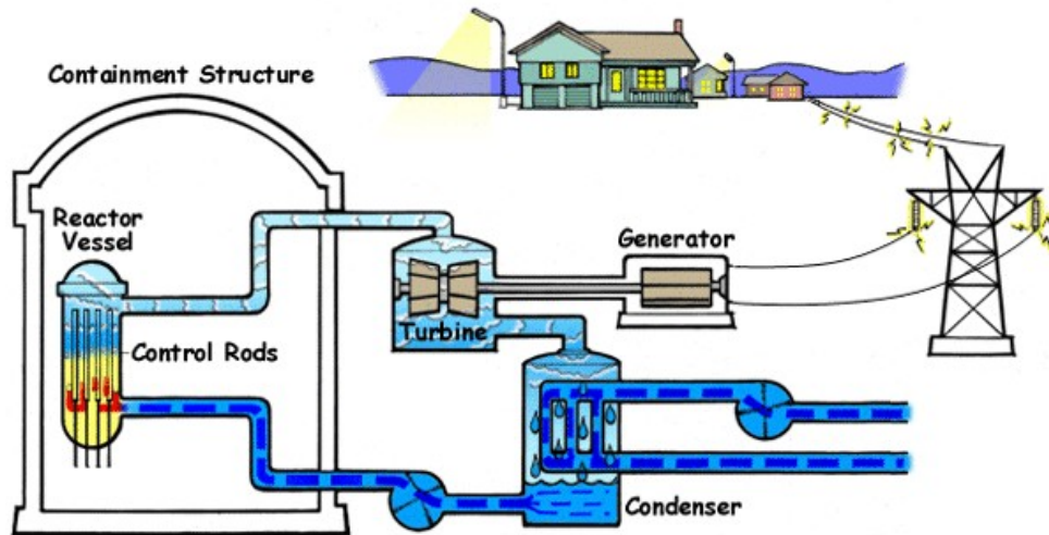
Figura 2.7 Reactor BWR
