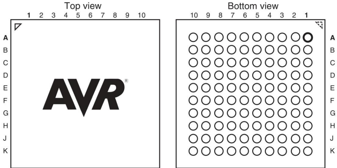
Figure 1-2. CBGA-pinout ATmega640/1280/2560
