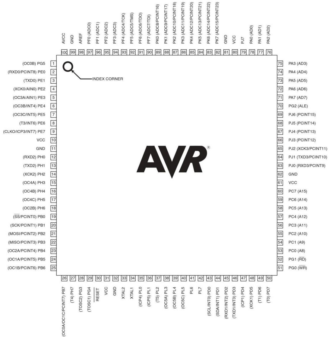
Figure 1-1. TQFP-pinout ATmega640/1280/2560
