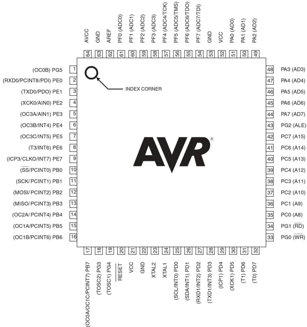
Figure 1-3. Pinout ATmega1281/2561
