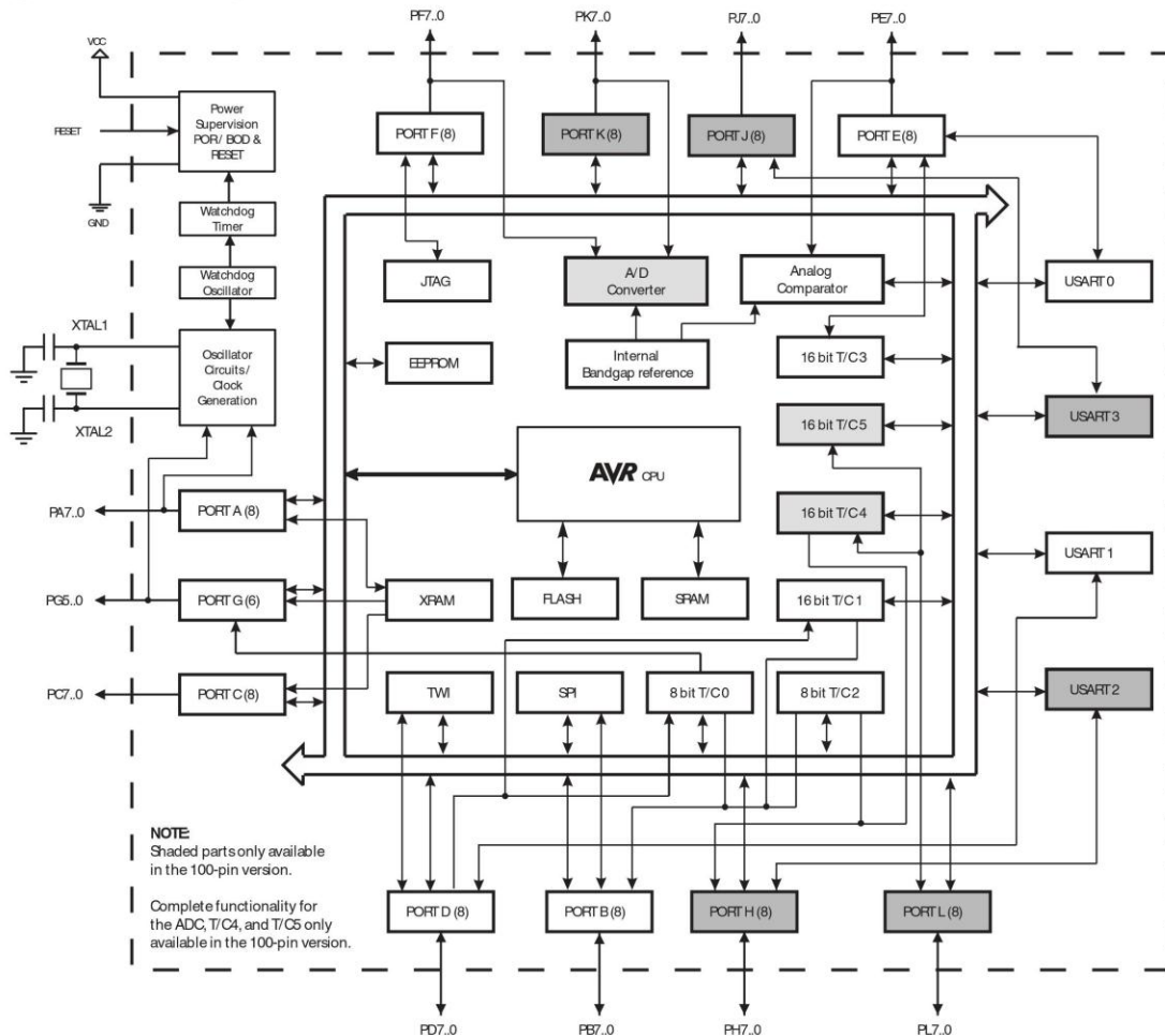
Figure 2-1. Block Diagram
