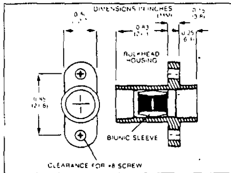
BICONIC MULTIMODE BULKHEAD OR IN LINE ADAPTER
